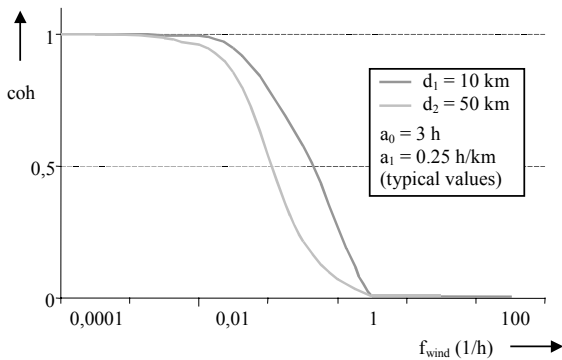
Figure 5 - Coherence \text{coh}(f_{wind}) of the wind velocity changing frequency f_{wind} for two distances d_1 and d_2
