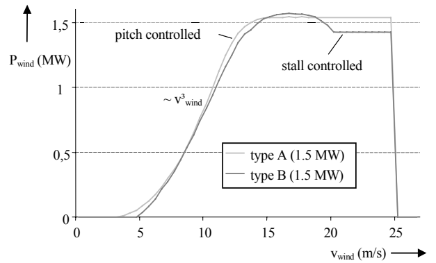
Figure 6. Electrical power generation of two wind energy converters dependent on the wind velocity.
