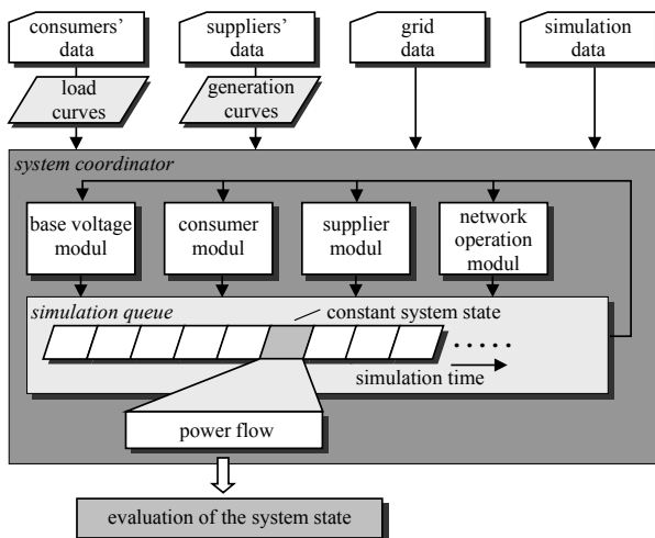
Figure7 - The simulation tool for steady-state voltage evaluation
