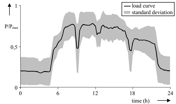
Figure 3 - A typical winter workday load curve of an industrial 2-shift consumer
