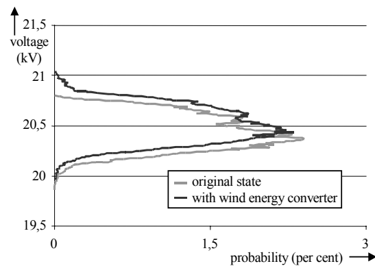
Figure 12 - Voltage states at node O
