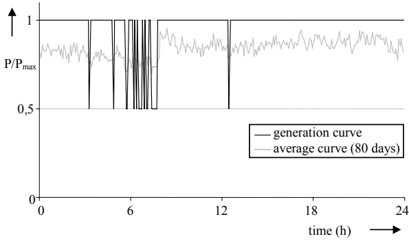
Figure 4 - A typical winter day generation curve of a 2-block power station
