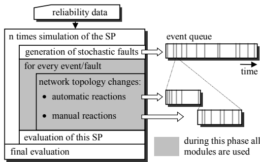
Figure 9 - Network operation considering faults
