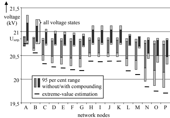
Figure 11 - Steady-state voltage evaluation
