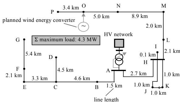
Figure 10 - The simulated rural 20 kV network
