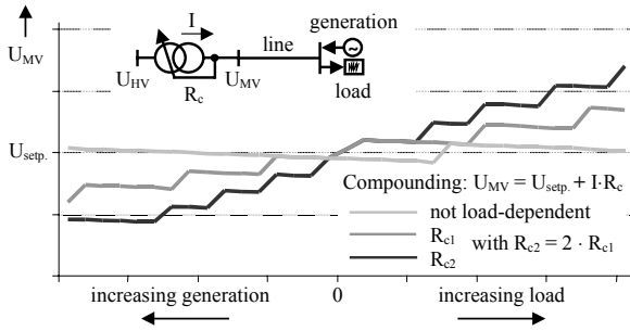
Figure 2 - Output voltage of a HV/MV transformer with a load-dependent voltage regulator
